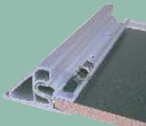
Marine plywood floorboards in an aluminium frame with tie-down rail system.
